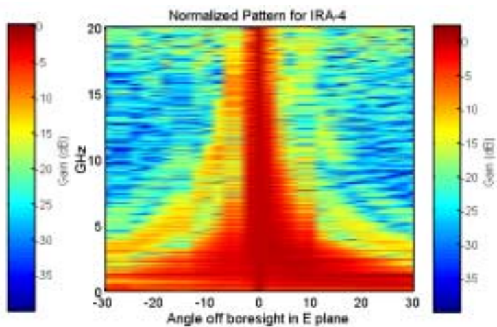
Figure 5.19. Pattern in the E plane. Angle is in degrees.
