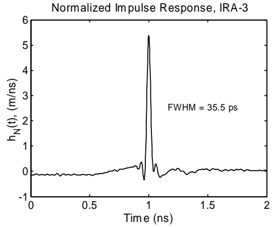
Figure 4.7. Normalized Impulse Response.
