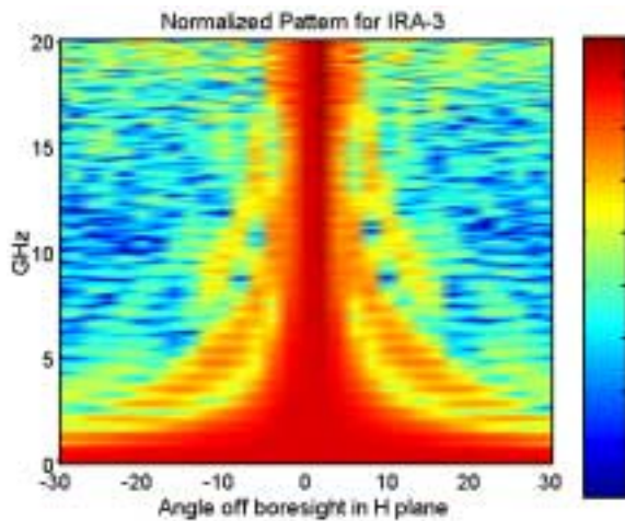
Figure 4.9. Pattern in the H plane. Angle is in degrees.
