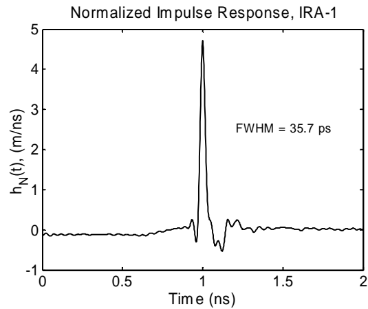
Figure 2.3. Normalized Impulse Response.
