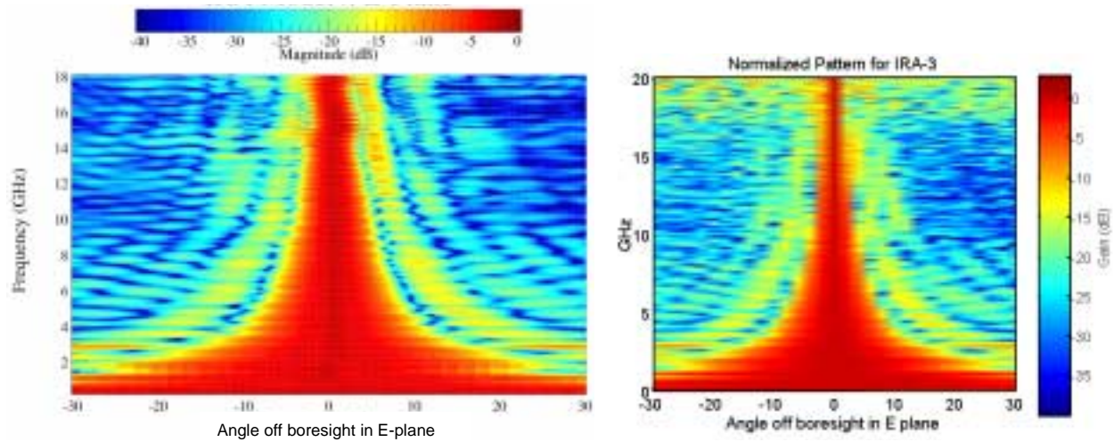
Figure 4.16. Pattern of the IRA-3 in the E plane, MRC left, FRI right. Angle is in degrees.
