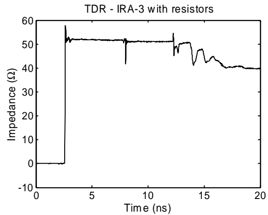
Figure 4.4. Four 200 \Omega metal film resistors in series/parallel.
