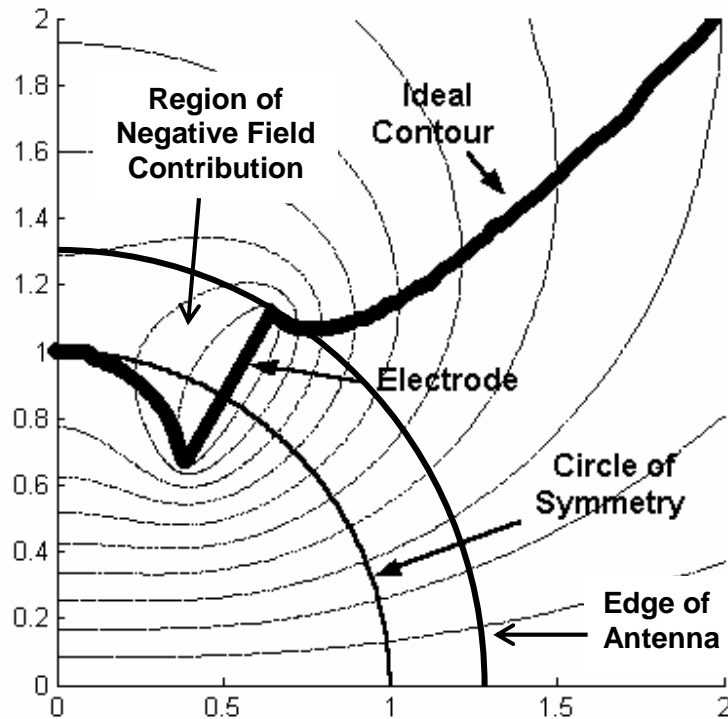
Figure 1.1. Sketch of the aperture fields of one-quarter of an IRA reflector.
