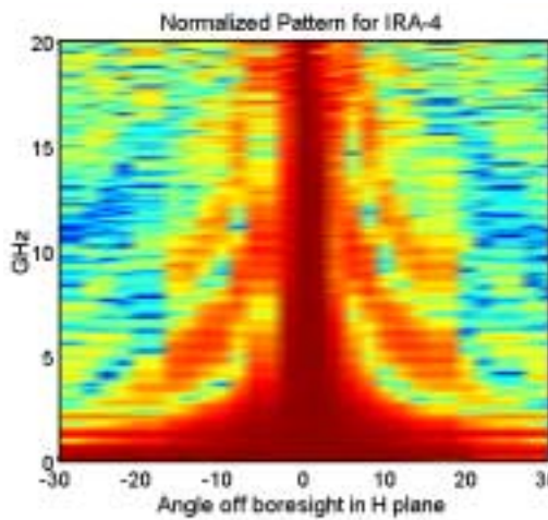
Figure 5.18. Pattern in the H plane. Angle is in degrees.
