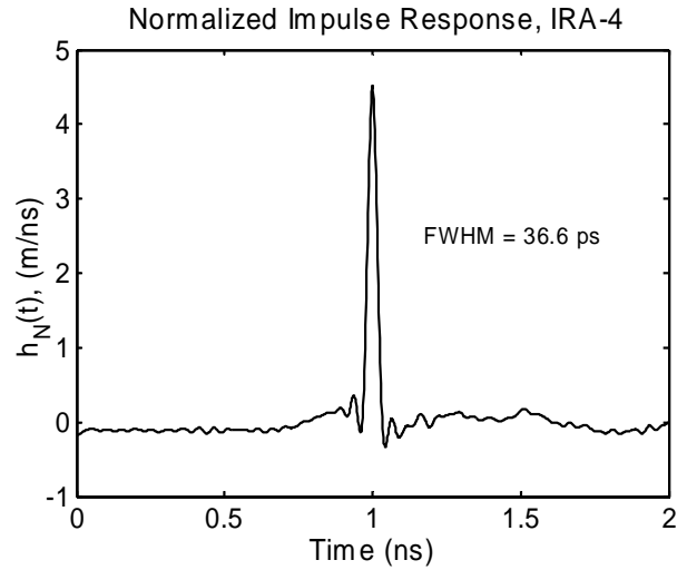
Figure 5.10. Normalized Impulse Response.
