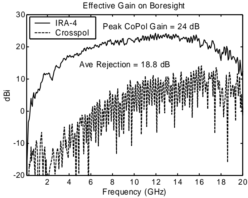
Figure 5.5. Effective gain of the IRA-4.
