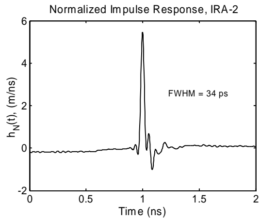
Figure 3.3. Normalized Impulse Response.
