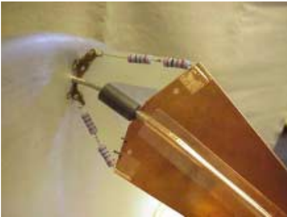
Figure 4.4. Four 200 \Omega metal film resistors in series/parallel.
