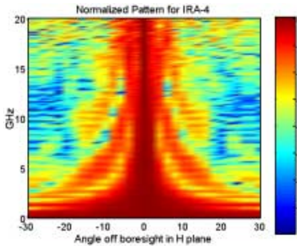
Figure 5.6. Pattern in the H plane. Angle is in degrees.
