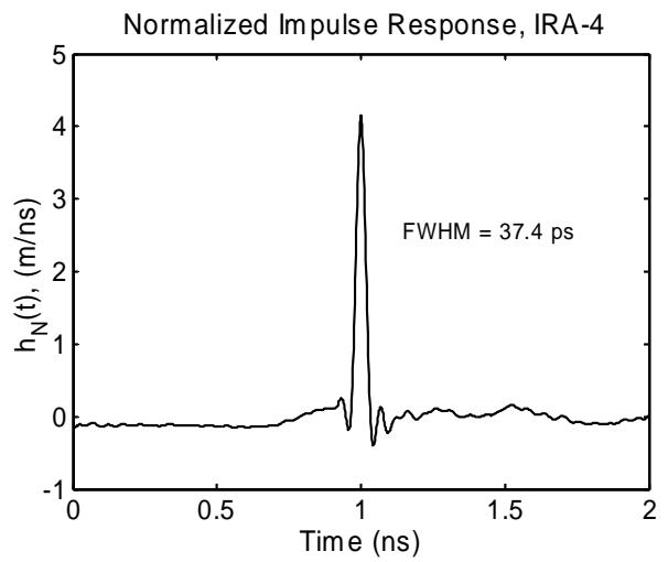
Figure 5.4. Normalized Impulse Response.
