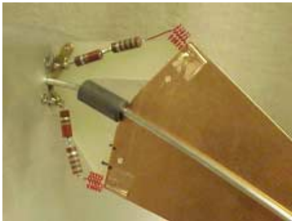
Figure 4.2. Two strings with a 10 turn figure 8 coil, a 180\ \Omega resistor, and a 220\ \Omega resistor.
