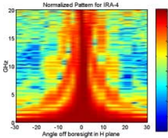
Figure 5.12. Pattern in the H plane. Angle is in degrees.
